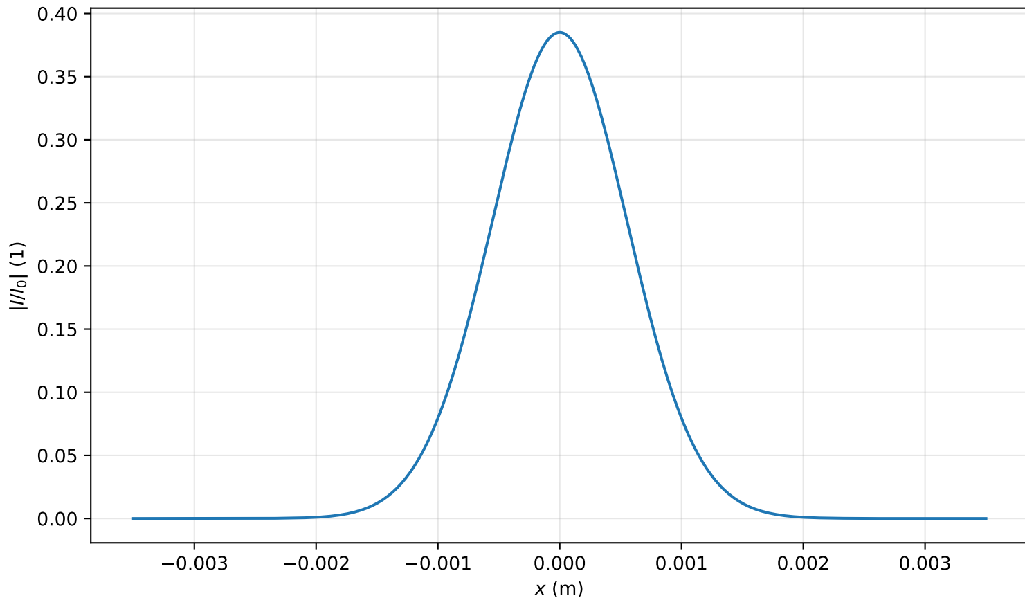
Intensity profile I(x, y = 0, z = 2.707m)/I_0 , P_{in}=0.1P_{cr} , artificial time
